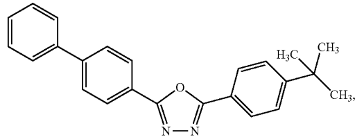
Oxadiazole-containing organic compound
