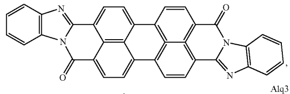
Perylene compound
