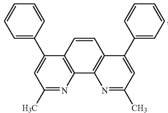
Phenanthroline-containing organic compound
