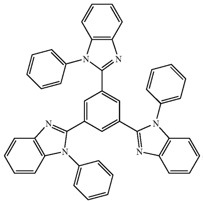
Phenanthroline-containing organic compound
